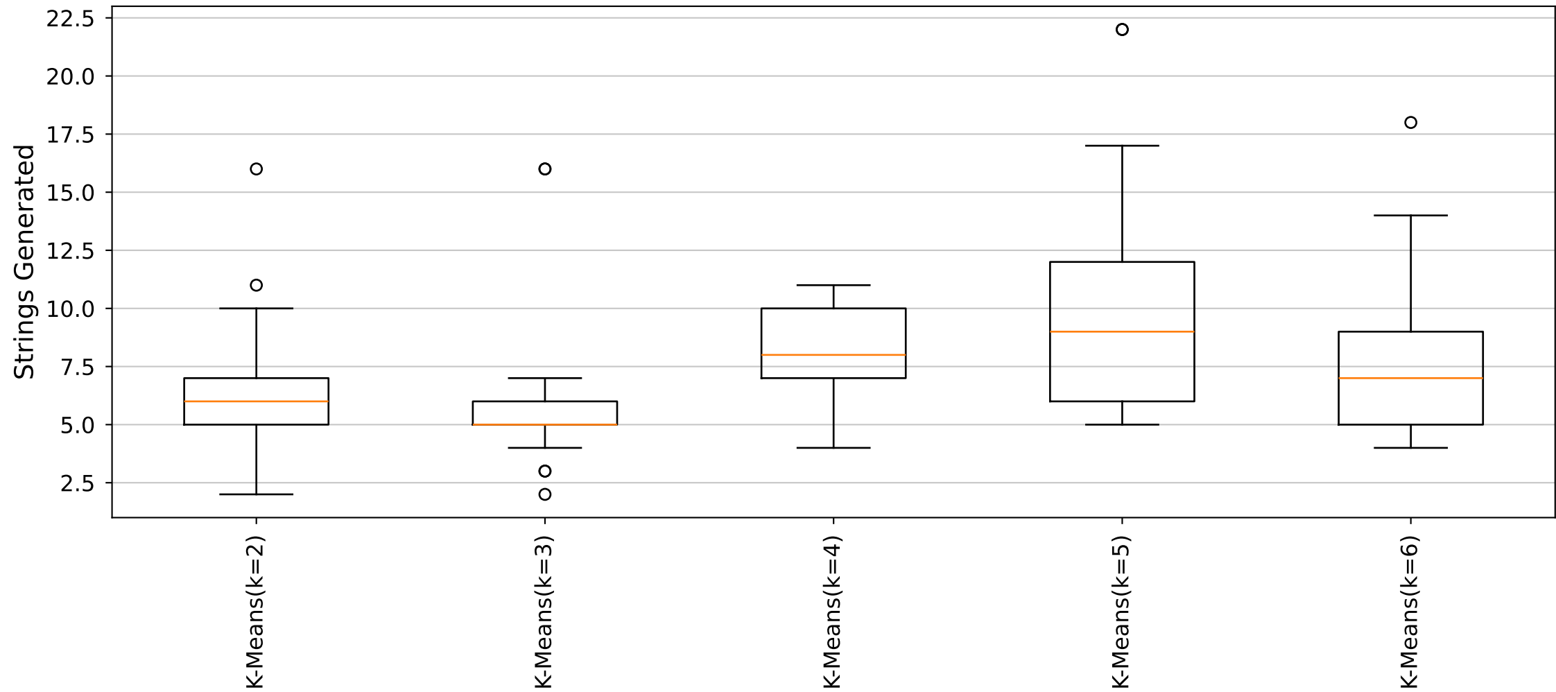
YARA Rules Strings Generated Distribution (Cluster27_Size6 dataset)
